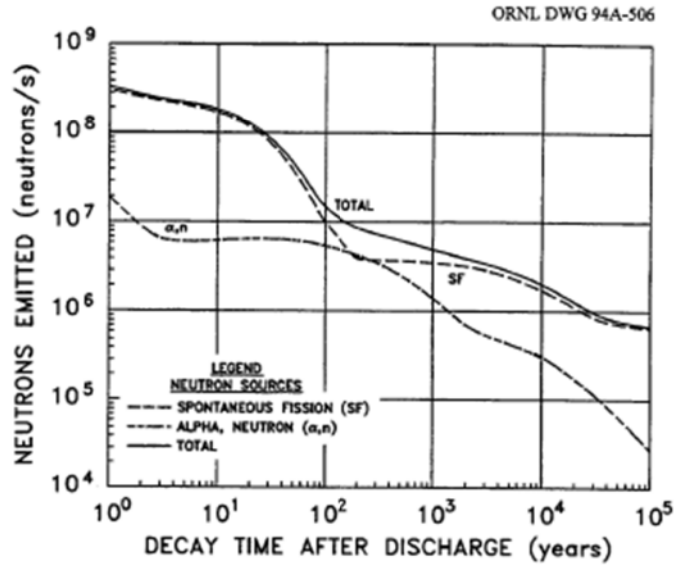
Fig. 9.2. Neutrons emitted by 1 metric ton of initial heavy metal (MTHM): PWR/33,000 MWd/MTU. Source: ref. 24.
