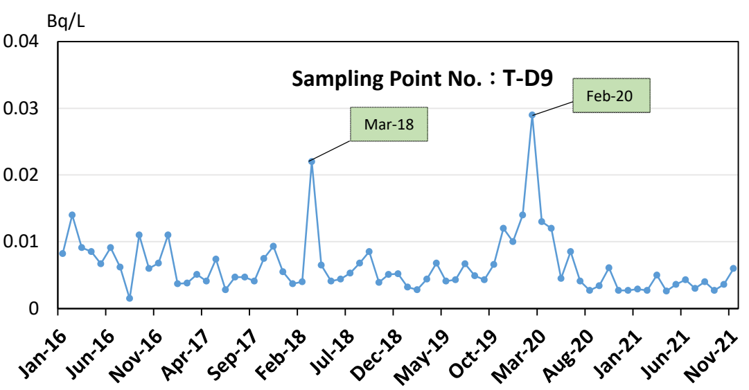
Concentration ranges of Cs-137 in sea-water around the Fukushima Daiichi NPS surveyed by the NRA
