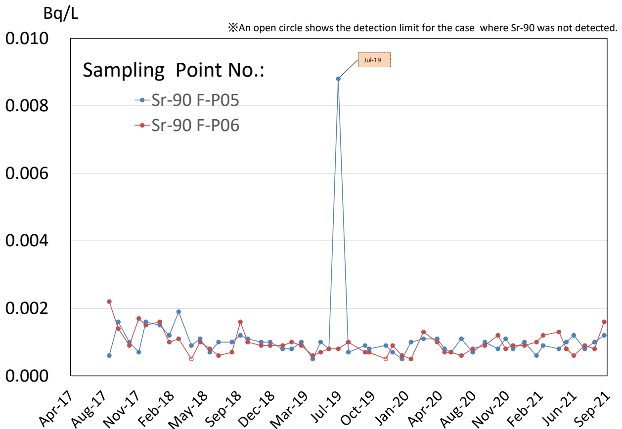
Concentration ranges of Sr-90 in sea-water around the Fukushima Daiichi NPS served by Fukushima prefecture
