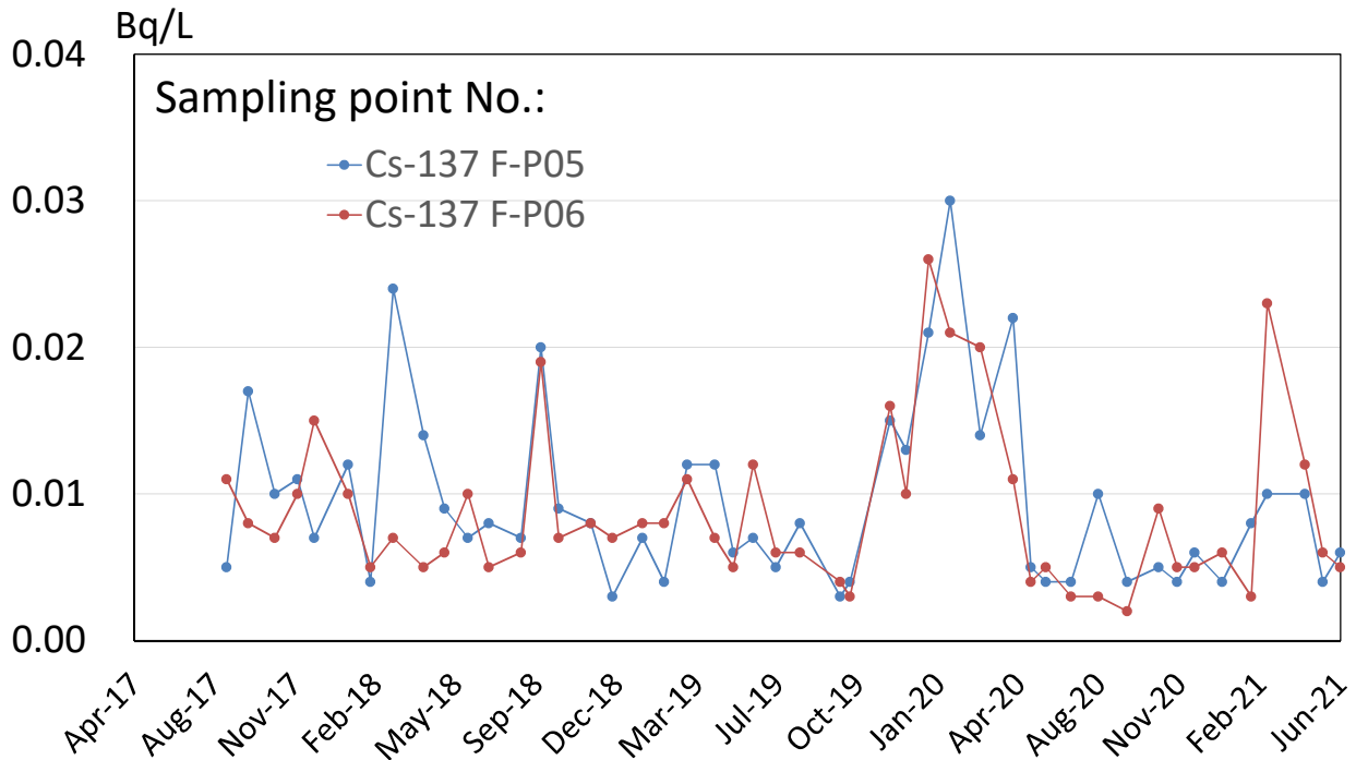
Concentration ranges of Cs-137 in sea-water around the Fukushima Daiichi NPS surveyed by Fukushima prefecture
