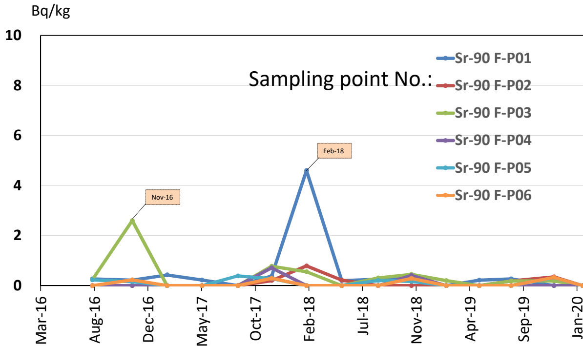
Concentration ranges of Sr-90 in sea-sediment near and around the Fukushima Daiichi NPS surveyed by Fukushima prefecture
