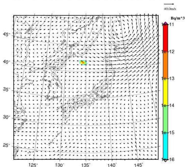
Xe-133 concentration at 3000m JST= 2016-09-10_15h00m
