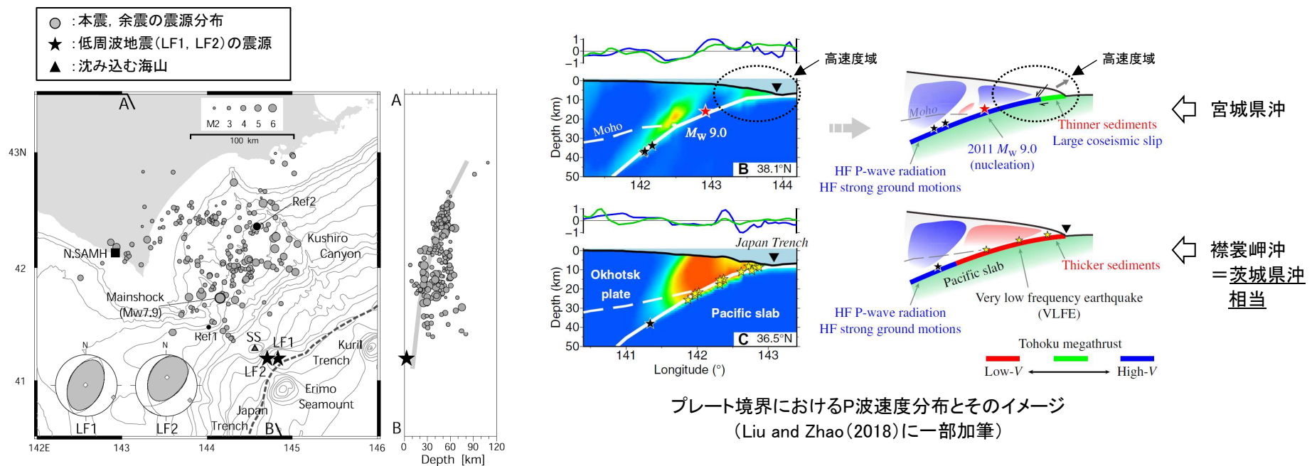
Fig. 1. (top) Hypocentral distribution of the main shock and aftershocks of the 2003 Tokachi-Oki earthquake and low-frequency (LF) earthquakes. Solid stars labeled LF1 and LF2 indicate the hypocentral location of LF events occurred at 3:37 am and 3:46 am, respectively. Aftershocks for the period of one month from the occurrence of the main shock are relocated by a homogeneous method with the fixed stations using stations of NIED Hi-net, JAMSTEC, Hokkaido University and JMA around the aftershock area. Well determined hypocenters with the horizontal error of less than 2 km and the vertical error less than 4 km are plotted on the bathymetric topography map. Focal mechanisms of the LF events estimated by the moment tensor inversion analysis are shown in the lower left corner. Solid circles labeled with Ref1 and Ref2 are the normal aftershocks whose seismograms are shown in Fig. 3 and Fig. 4 as references compared with the LF events. The solid square symbol is the location of the station N.SAMH where observed seismograms are plotted in the Fig. 2 and Fig. 3. The triangle symbol labeled with SS indicates the swell produced by a subducted seamount in the inner trench slope. The dashed line indicates the axis of the Kuril Trench and the Japan Trench. Along the profile of AB, the cross sectional view of aftershocks is shown in the right side. Gray bold line is the plate boundary along the AB profile proposed by Earthquake Research Committee (2003). (Bottom) Time sequence of aftershock activity for 2003 Tokachi-Oki earthquake and LF earthquakes. Earthquakes listed in JMA catalog located in the rectangle area shown in top panel are plotted with the time duration of ten days. Circles indicate earthquakes, of which the magnitude is greater than 5.5. LF events are indicated by star symbols.
