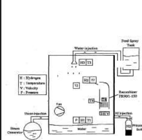
fig. 1. Experimental apparatus
