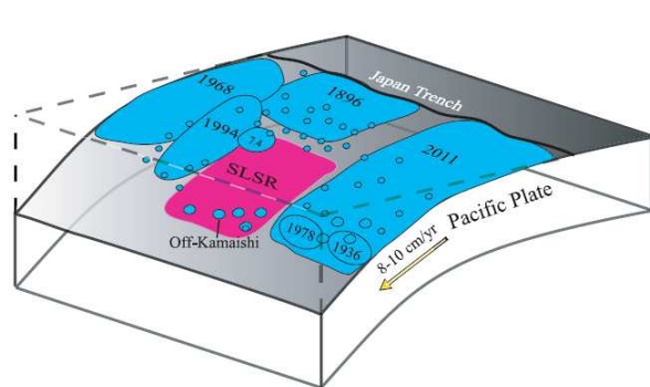
Figure 12. Schematic map of the Japan megathrust fault showing the distribution of rupture zone of historic large events and the 2011 Tohoku earthquake (large blue regions), and aftershocks (small blue regions) along the megathrust from Japan Trench. We plot the southern end of the 1896 rupture zone as extending to about 39°N, north of the aseismic zone seen in Figure 2e, consistent with the southern extent of the tsunami model of Aida [1977] and the region of strong inundation on the Iwate coast indicated by Hatori [1974]. The convergence velocity of the Pacific Plate is indicated by a yellow arrow. The magenta region highlights the SLSR on the megathrust. The SLSR is largely aseismic, but does have modest-size patches of seismicogenic regions down-dip, including the off-Kamaishi repeater zone. The shallower portion of the SLSR is almost devoid of moderate-size thrust events, but seismic activity is high in the 1896 rupture zone region further updip.
