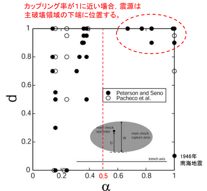
Fig. 1. The relative hypocentral depth d versus the seismic coupling coefficient α obtained for large interplate earthquakes at subduction zones (Table 1). Solid and open circles stand for α values from Peterson and Seno [7] and from Pacheco et al. [15], respectively. When α is estimated to be greater than 1 (Table 1), it is reduced to 1. The relative hypocentral depth d is defined by D / W , where D is the distance from the trenchward edge of the rupture area to the epicenter and W is the width of the rupture area in the direction perpendicular to the trench axis (inset).
