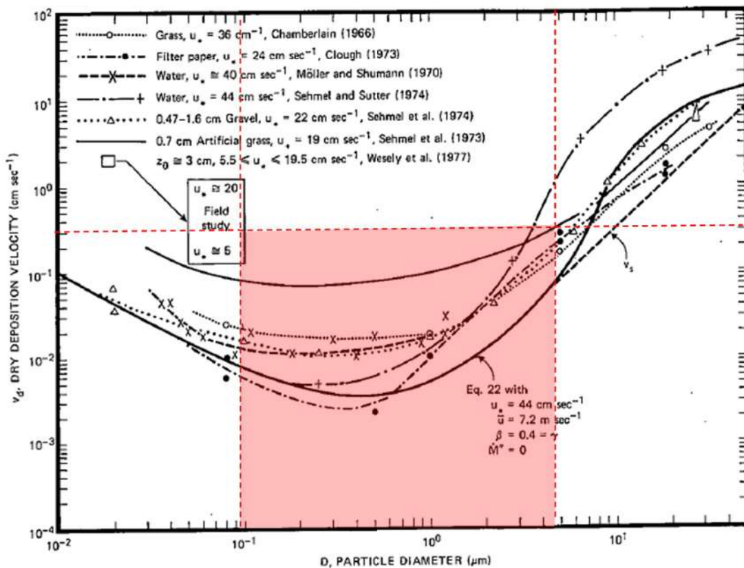
Fig. 4 Dry deposition velocity as a function of particle size. Data were obtained from a number of publications. 1)~5) The theoretical curve appropriate for a smooth surface is shown for comparison. Note that the theoretical curve is strongly dependent on the value for u_* and that Eq. 22 does not contain a parameterization for surface roughness. For a preliminary study of the effect of surface roughness and other factors, see Ref. 5.
