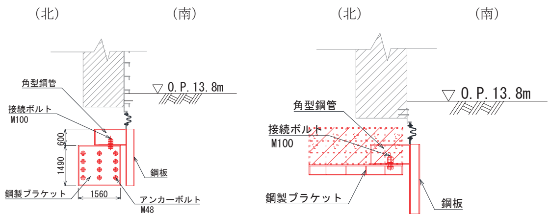
(断面図, 2-2)
