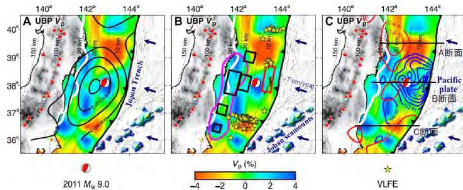
Fig. 4. V_p tomography and characteristics of the 2011 Tohoku-oki earthquake. The colors in (A) to (C) show V_p tomography along the UBPs obtained by this study. Black bold contour lines in (A) denote the back-slip rate (5). In (B), the yellow stars mark epicenters of very low frequency earthquakes (VLFs) (24); the red rectangle denotes a slow slip event (22) preceding the 2011 Tohoku-oki earthquake; the black rectangles show locations of coseismic strong ground motions (39); the magenta contour line marks the site of coseismic high-frequency P-wave radiation with a relatively low seismic moment during the 2011 Tohoku-oki earthquake (40); and the black short lines near the trench indicate seafloor traces of normal faults (34). The blue and red contour lines in (C) denote the coseismic slip (7) and the afterslip (43), respectively. The other labeling is the same as that in Fig. 2.
