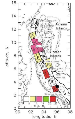
Tanioka et al. (2006) (46)
