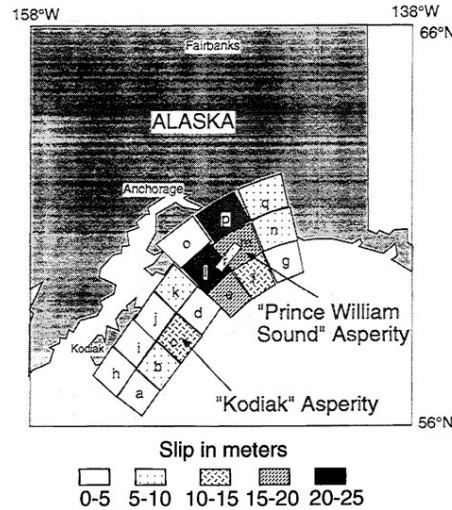
Johnson et al. (1996) (44)
