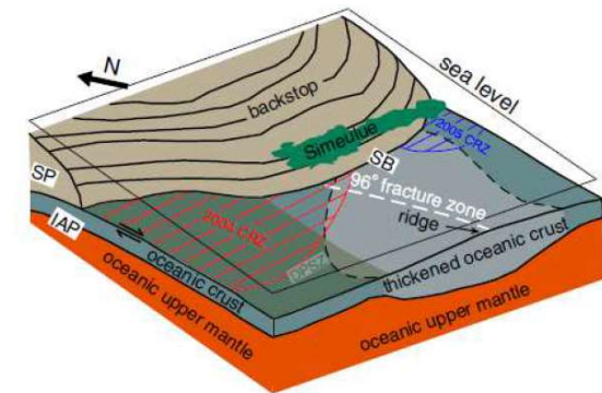
Figure 4. Cartoon illustrating the segmentation of the 2004-2005 megathrust rupture in the Sumatra subduction zone around Simeulue Island. The accretionary complex removed for simplicity. CRZ: coseismic rupture zone; SP: Sunda plate. Other labels same as in Figures 2 and 3.
