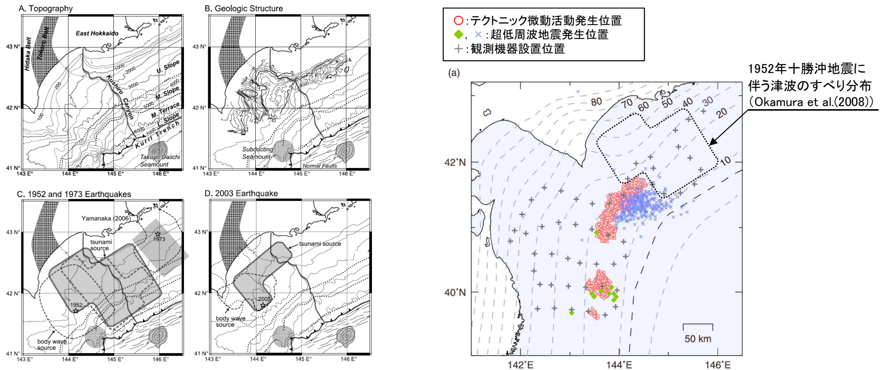
Figure 5. Comparison of topography, geologic structure, earthquake and tsunami sources, and geophysical data. (a) Bathymetric contour map, (b) depth contour map at the base of Pliocene sediments (contour interval of 0.2 s in two-way travelttime), (c) and (d) seismic and tsunami sources defined as the areas with slip larger than 1 m for Yamanaka and Kikuchi [2003], Tanioka et al. [2004], and Satake et al. [2006] and 1.2 m for Yagi [2004], (e) magnetic anomaly [Joshima, 2005] (contour interval of 50 nT), and (f) gravity anomaly [Joshima, 2005] (contour interval of 10 mGal).
