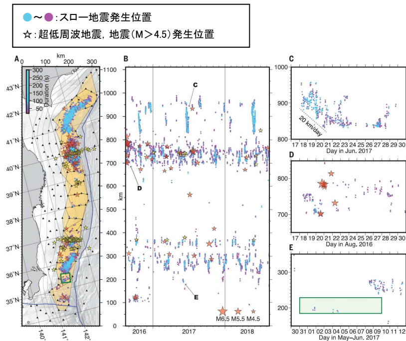
Fig. 1. Tremor activity in the Japan Trench. (A) Epicenters of the tectonic tremors. Dots indicate the epicenters of the tremors, which are colored according to their duration (see the color scale). Yellow and red stars are VLFs and M > 4.5 ordinary earthquakes, respectively, with the ordinary earthquake epicenters taken from the Japan Meteorological Agency (JMA) catalog. Black triangles are S-net observatories. The green square denotes the June 2017 SSE that was detected by our GNSS analysis.
