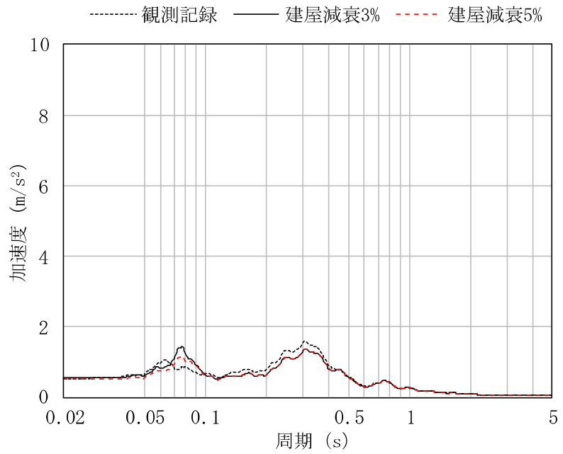
(c) 鉛直方向 4F (T.M.S.L. 31.7m, h = 5%)
