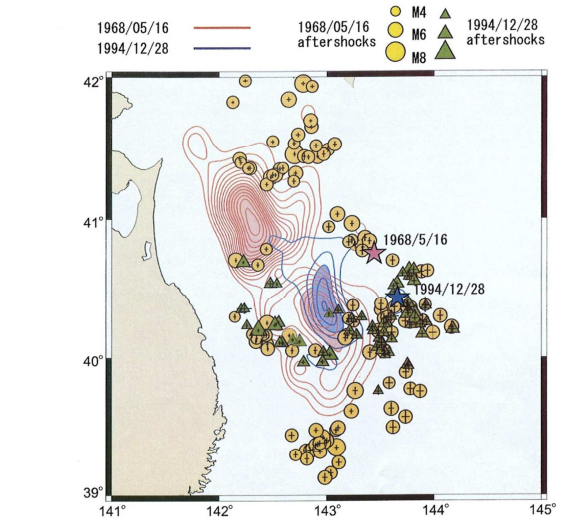
Fig. 13. Comparison between the moment release and the aftershocks both in the 1968 Tokachi-oki and the 1994 Sanriku-oki events. Red lines indicate the moment release of the 1968 event, and blue lines indicate that of the 1994 event. The contour interval is 3 \times 10^{16} [Nm/km 2 ]. Circles denote the aftershocks of the 1968 event, and triangles those of the 1994 event.
