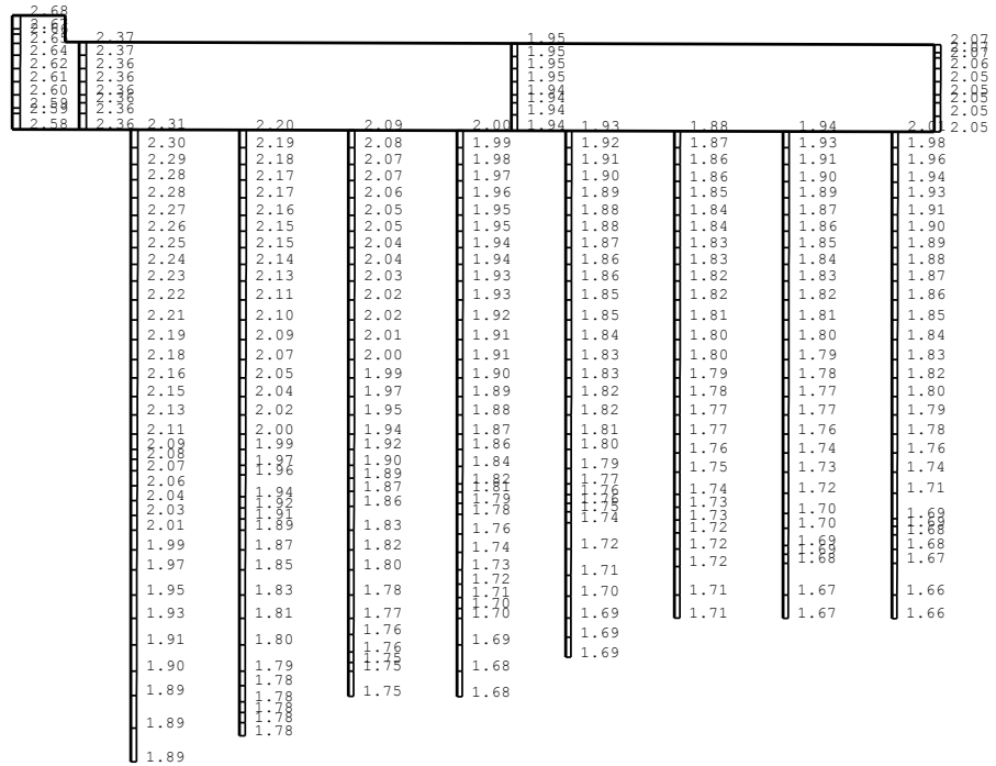
(b) Sd-2NS, 鉛直
