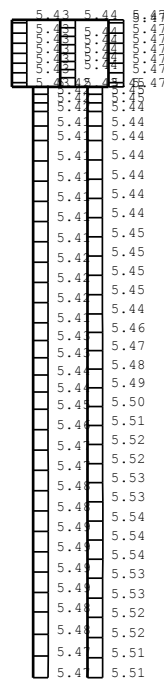
(b) Ss-1-+, 鉛直
