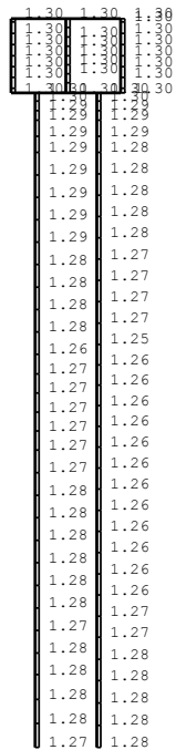
(b) Sd-4NS, 鉛直
