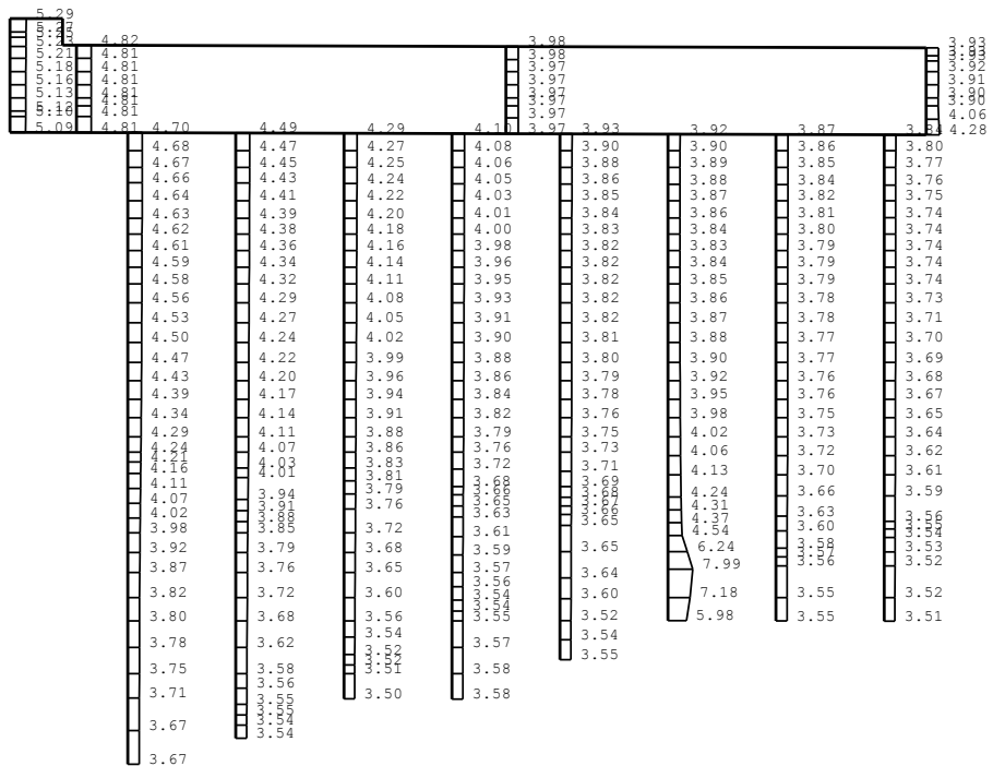
(b) Ss-2EW, 鉛直
