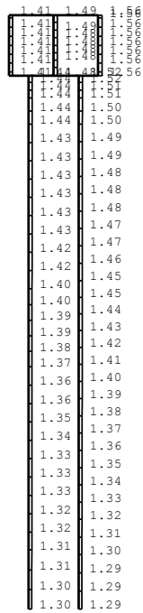
(b) Sd-7NS, 鉛直
